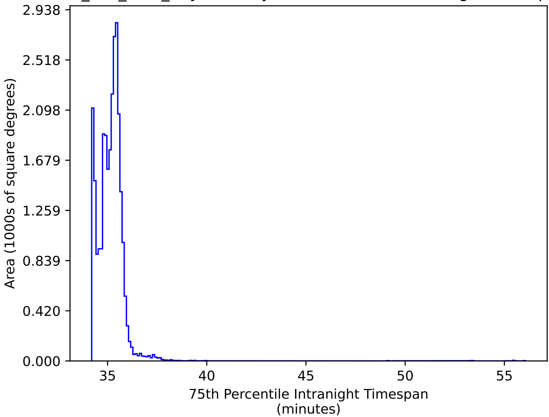
smc_lmc_v3.3_10yrs All sky: 75th Percentile Intranight Timespan
