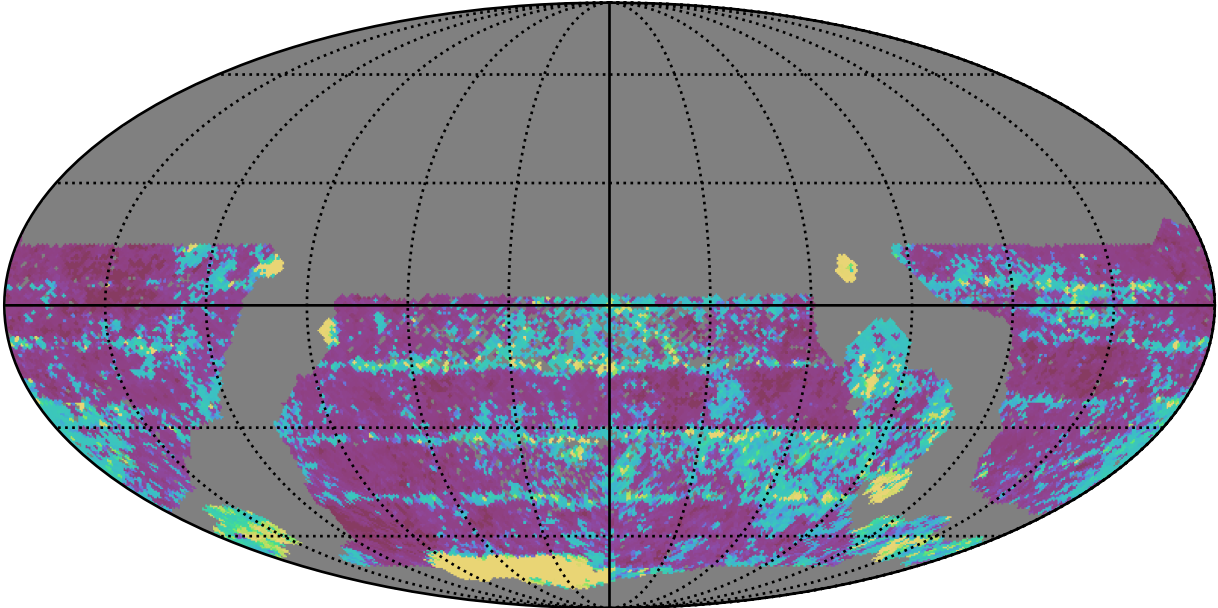
smc_lmc_v3.3_10yrs WFD z band: 20thPercentile Inter-Night Gap
