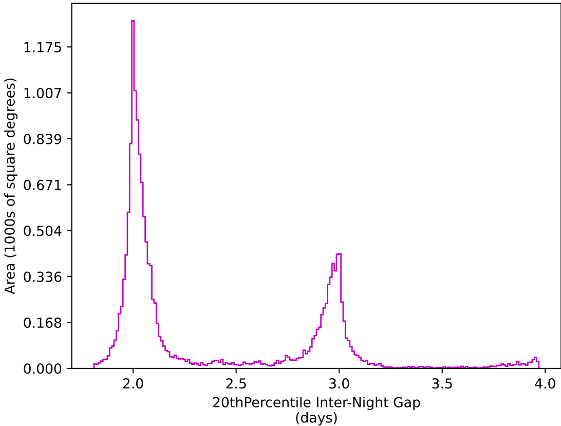
smc_lmc_v3.3_10yrs WFD z band: 20thPercentile Inter-Night Gap
