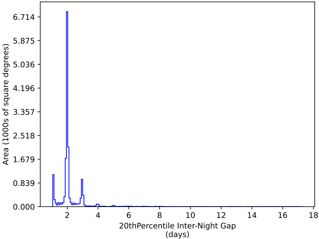
smc_lmc_v3.3_10yrs WFD y band: 20thPercentile Inter-Night Gap
