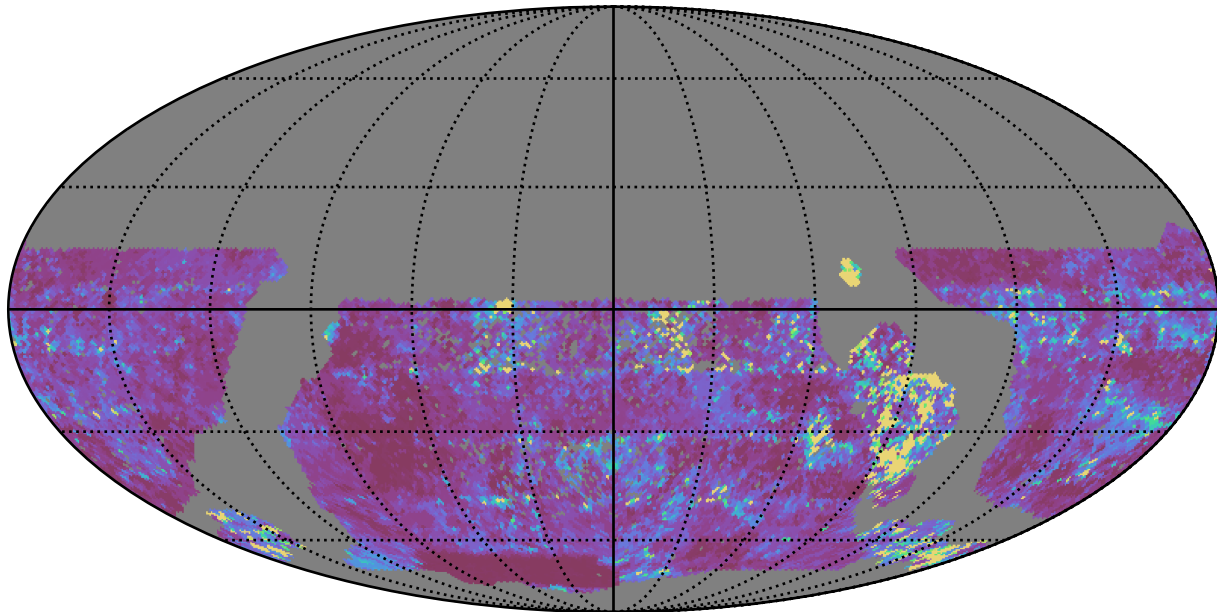
smc_Imc_v3.3_10yrs WFD u band: 20thPercentile Inter-Night Gap
