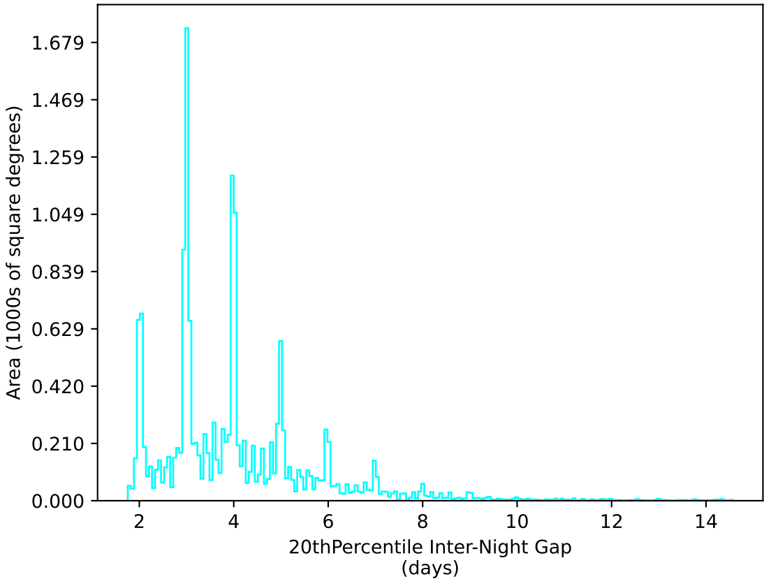
smc_lmc_v3.3_10yrs WFD u band: 20thPercentile Inter-Night Gap
