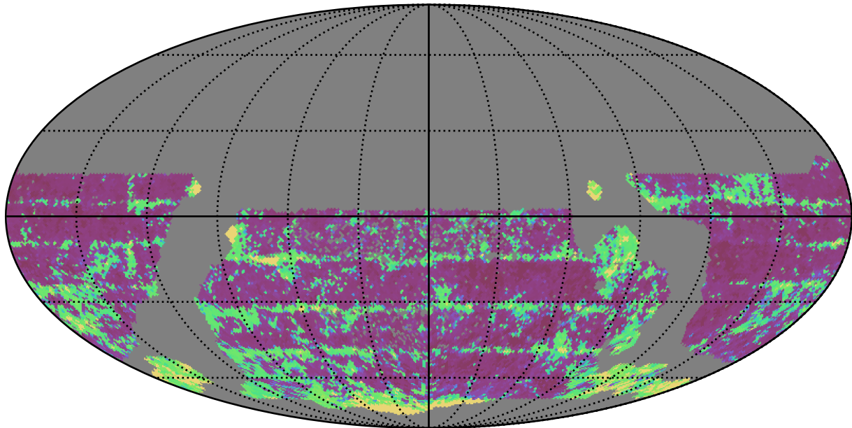
smc_lmc_v3.3_10yrs WFD i band: 20thPercentile Inter-Night Gap
