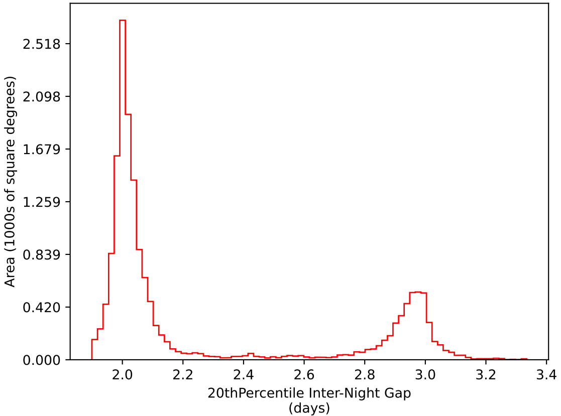
smc_lmc_v3.3_10yrs WFD i band: 20thPercentile Inter-Night Gap
