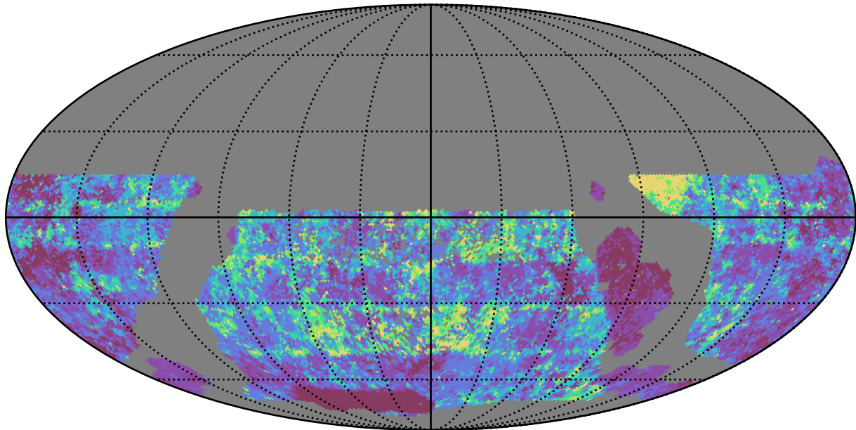
smc_Imc_v3.3_10yrs WFD g band: 20thPercentile Inter-Night Gap
