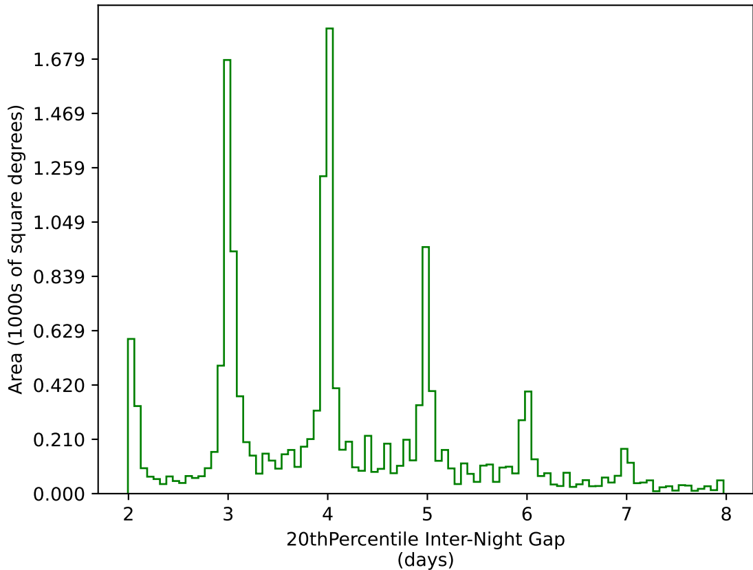
smc_lmc_v3.3_10yrs WFD g band: 20thPercentile Inter-Night Gap
