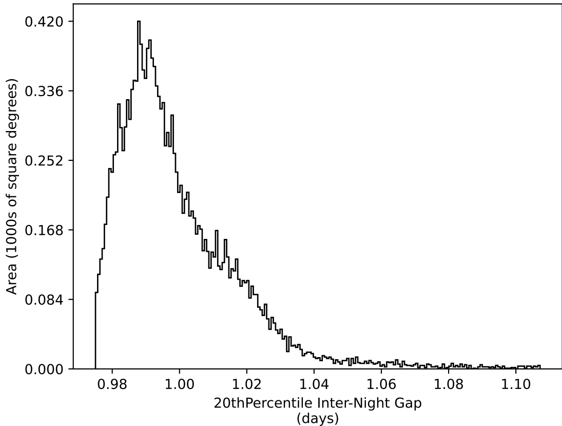
smc_lmc_v3.3_10yrs WFD all bands: 20thPercentile Inter-Night Gap
