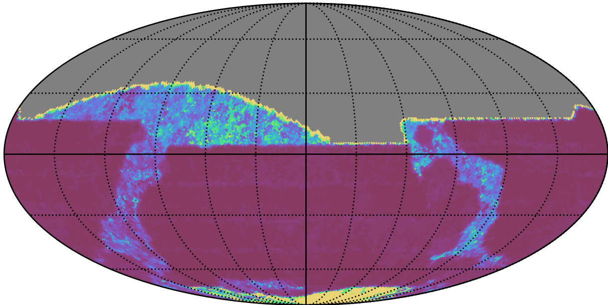
smc_lmc_v3.3_10yrs All sky z band: 20thPercentile Inter-Night Gap
