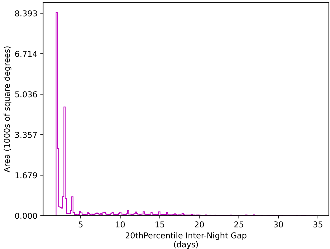
smc_lmc_v3.3_10yrs All sky z band: 20thPercentile Inter-Night Gap
