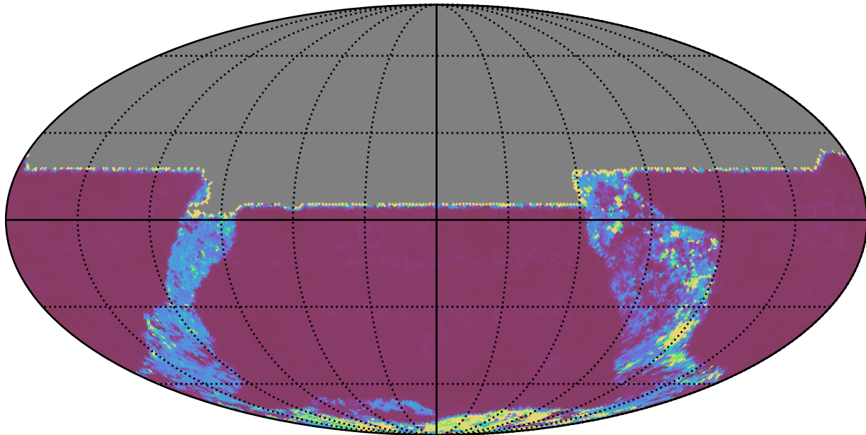
smc_lmc_v3.3_10yrs All sky y band: 20thPercentile Inter-Night Gap
