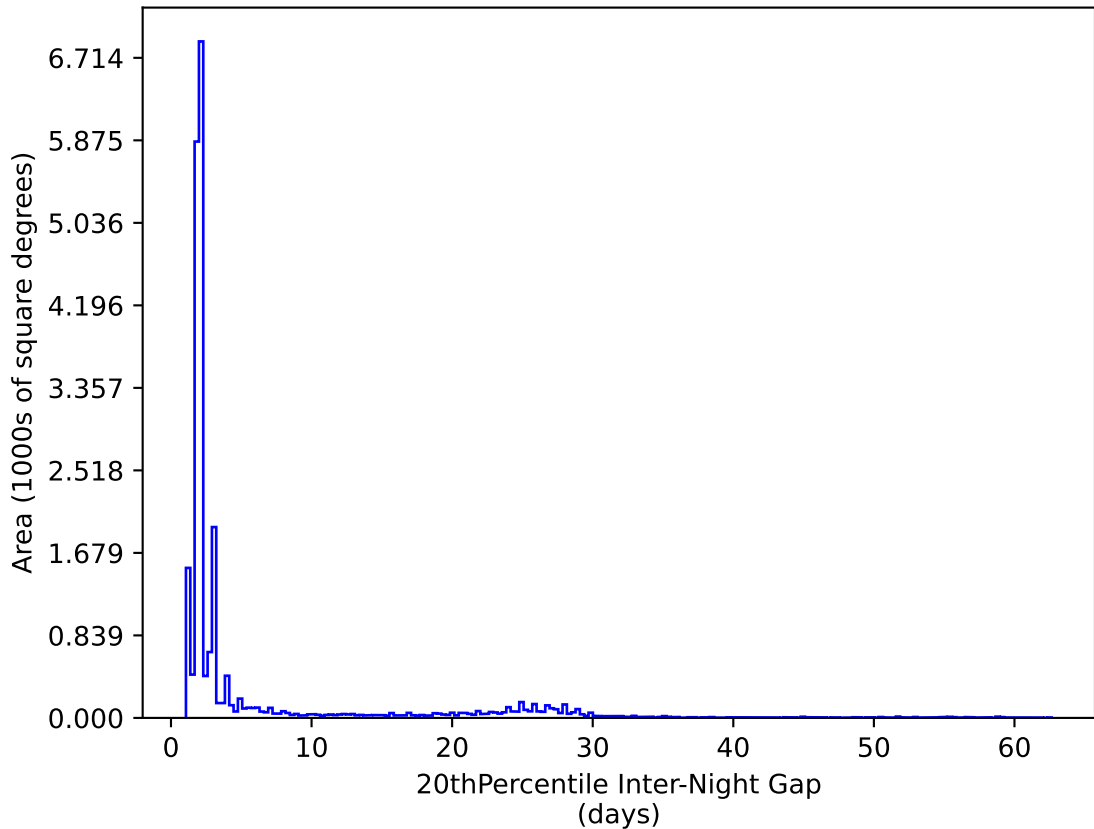
smc_lmc_v3.3_10yrs All sky y band: 20thPercentile Inter-Night Gap
