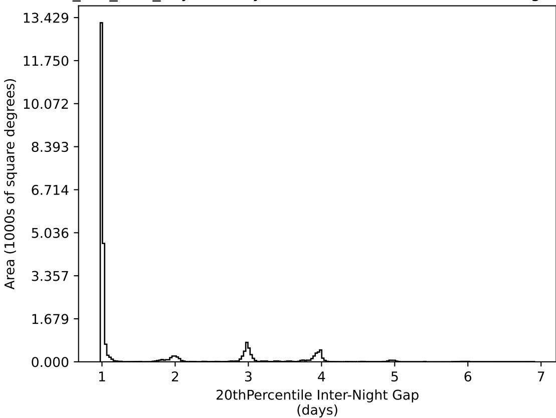
smc_Imc_v3.3_10yrs All sky all bands: 20thPercentile Inter-Night Gap
