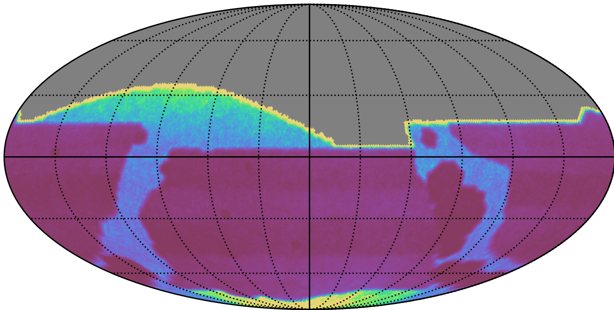
smc_lmc_v3.3_10yrs : properMotion
