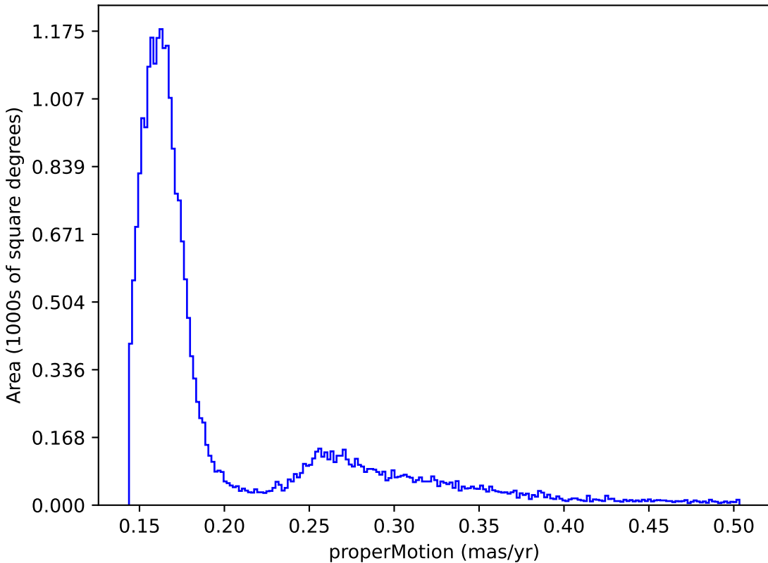
smc_lmc_v3.3_10yrs : properMotion
