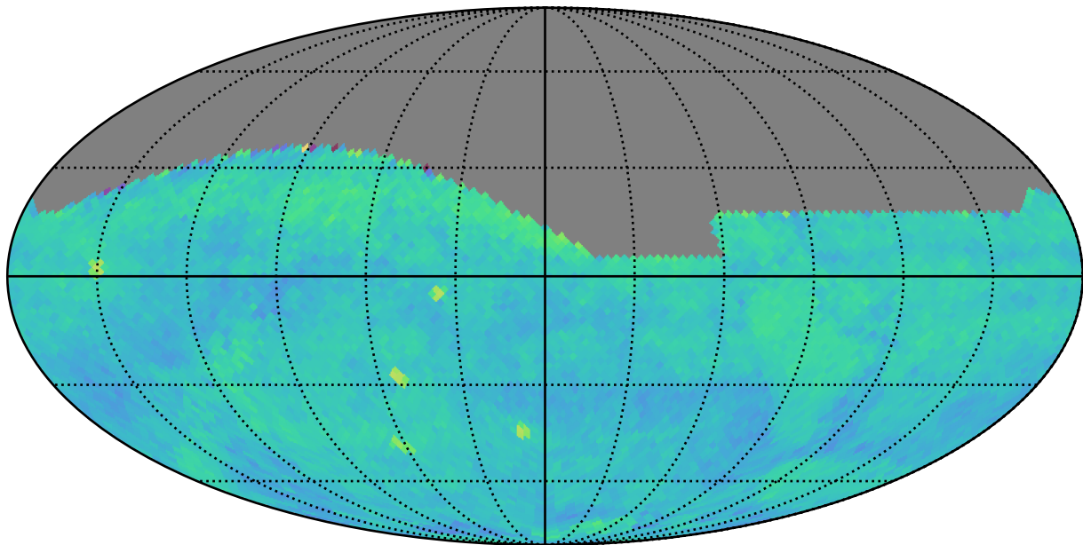
smc_lmc_v3.3_10yrs (g or r or i): PairFraction
