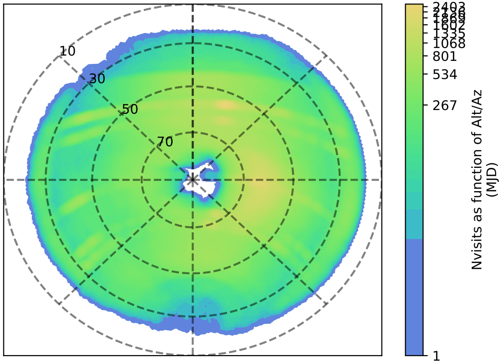
smc_lmc_v3.3_10yrs z: Nvisits as function of Alt/Az
