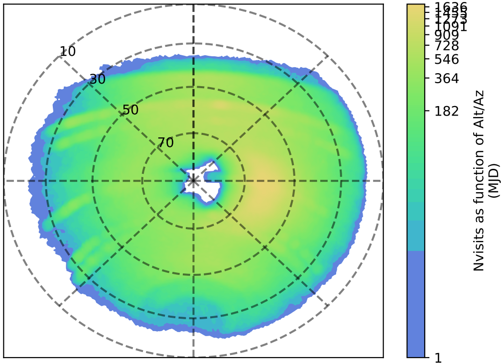
smc_lmc_v3.3_10yrs y: Nvisits as function of Alt/Az
