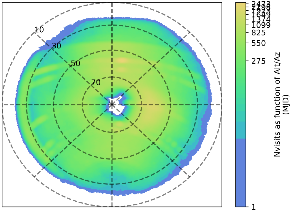
smc_lmc_v3.3_10yrs r: Nvisits as function of Alt/Az
