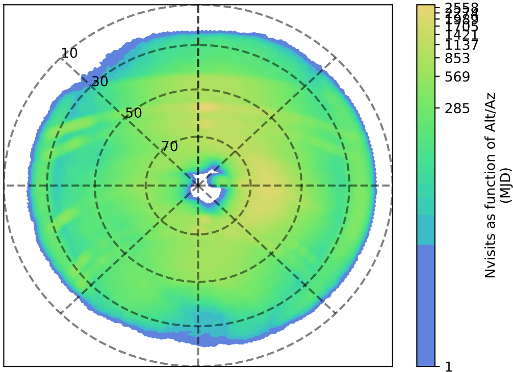
smc_lmc_v3.3_10yrs i: Nvisits as function of Alt/Az
