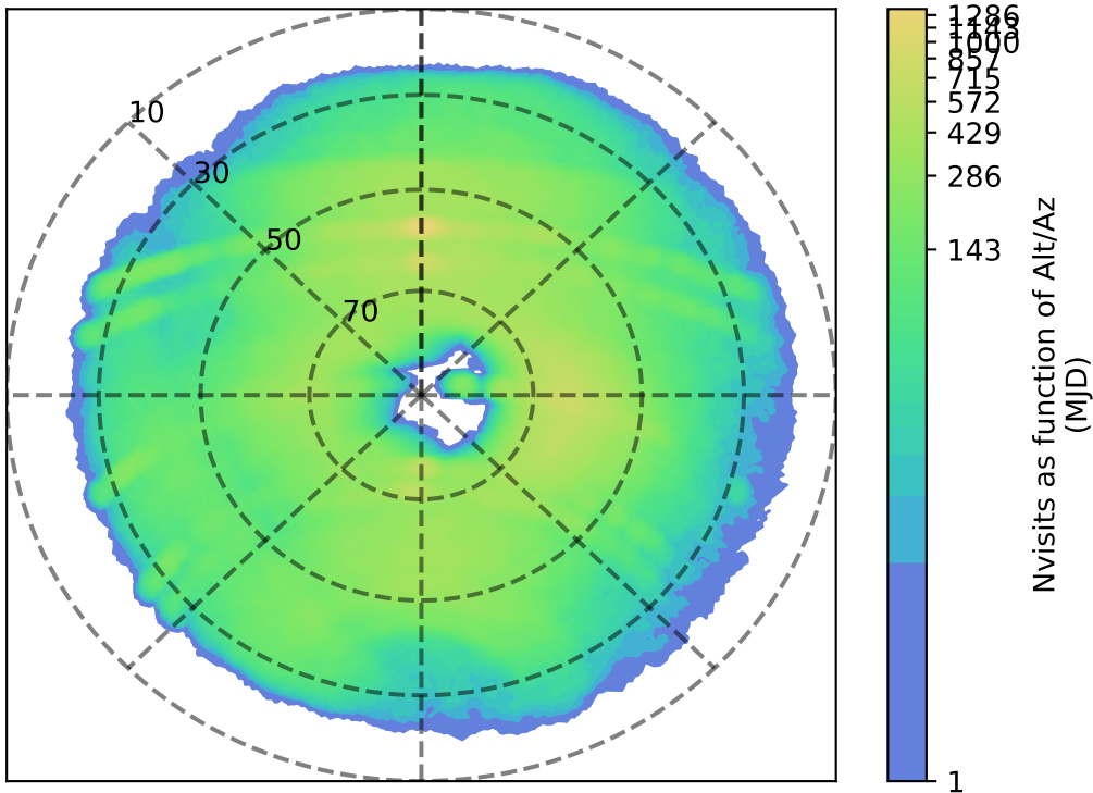
smc_lmc_v3.3_10yrs g: Nvisits as function of Alt/Az
