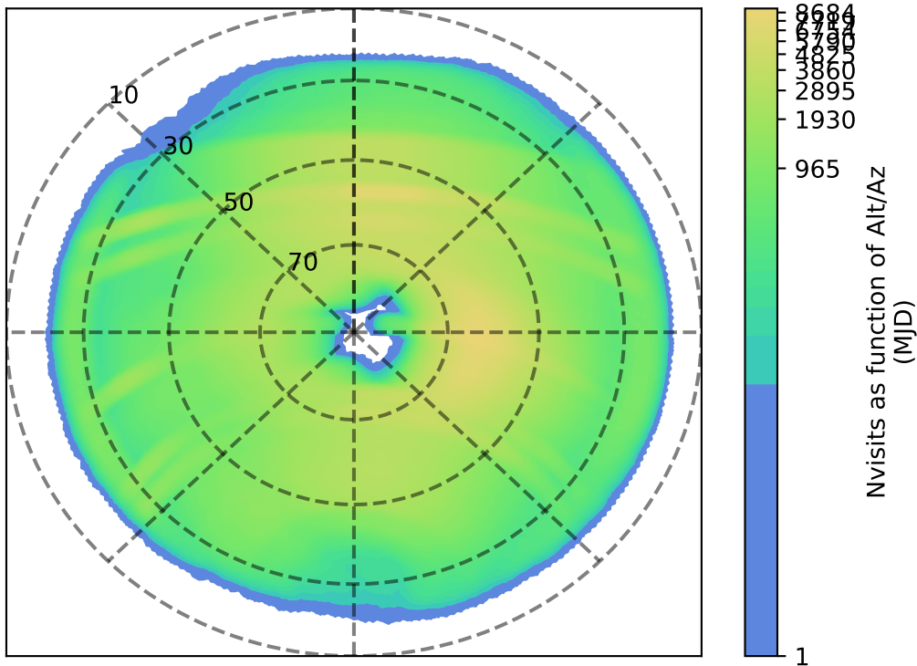
smc_lmc_v3.3_10yrs : Nvisits as function of Alt/Az
