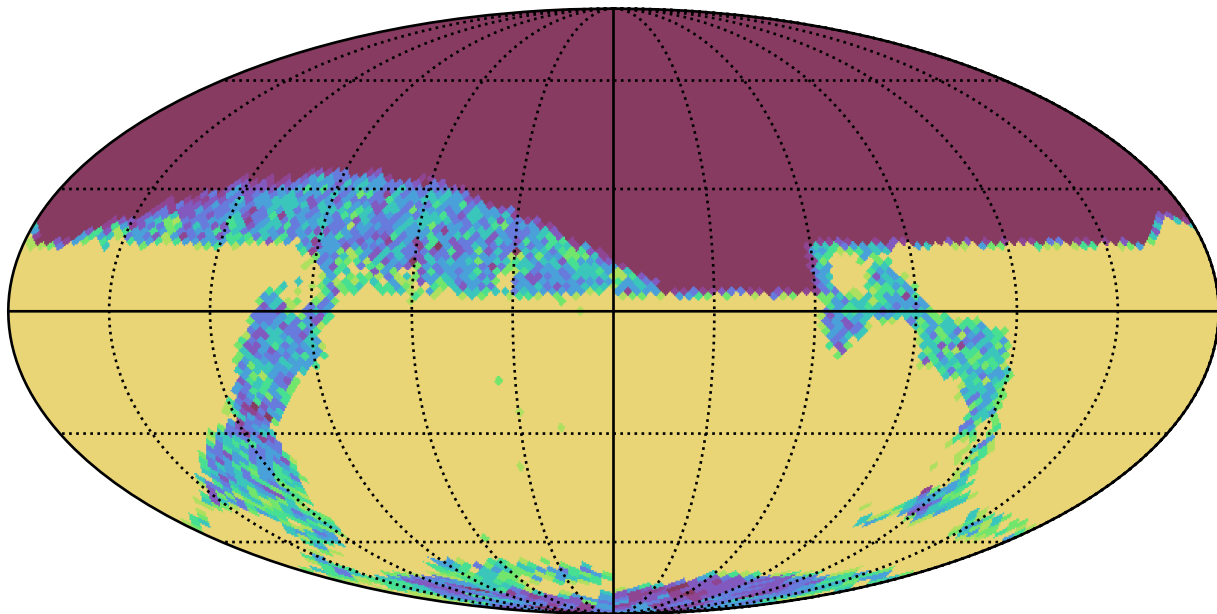
smc_lmc_v3.3_10yrs z and night < 365: N year 1
