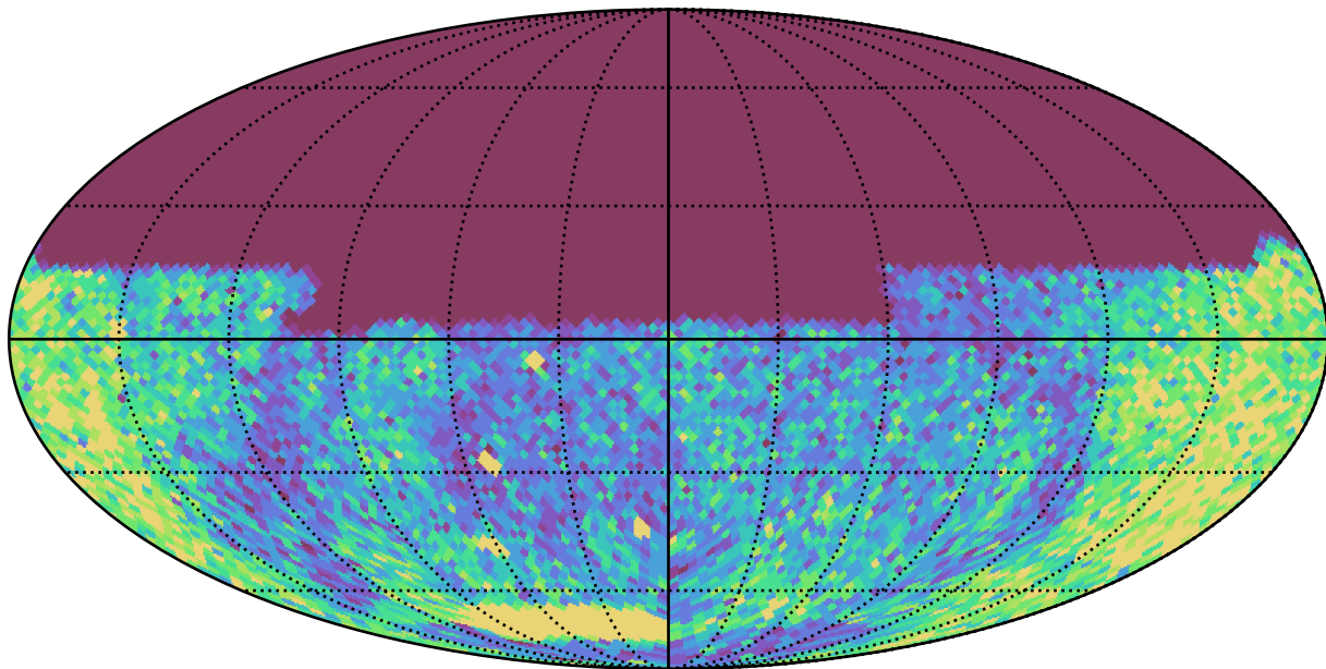
smc_lmc_v3.3_10yrs u and night < 365: N year 1
