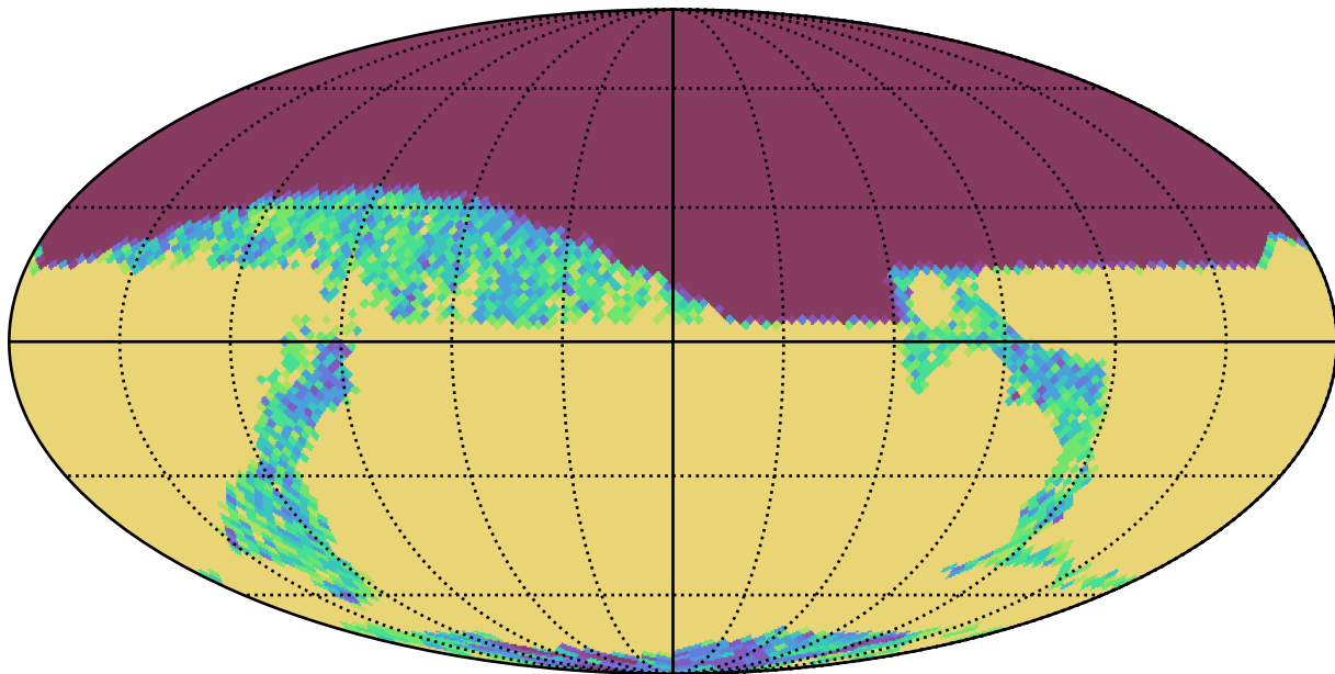
smc_lmc_v3.3_10yrs i and night < 365: N year 1
