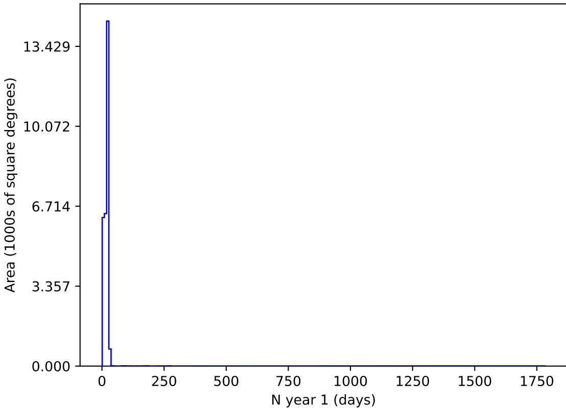
smc_lmc_v3.3_10yrs i and night < 365: N year 1
