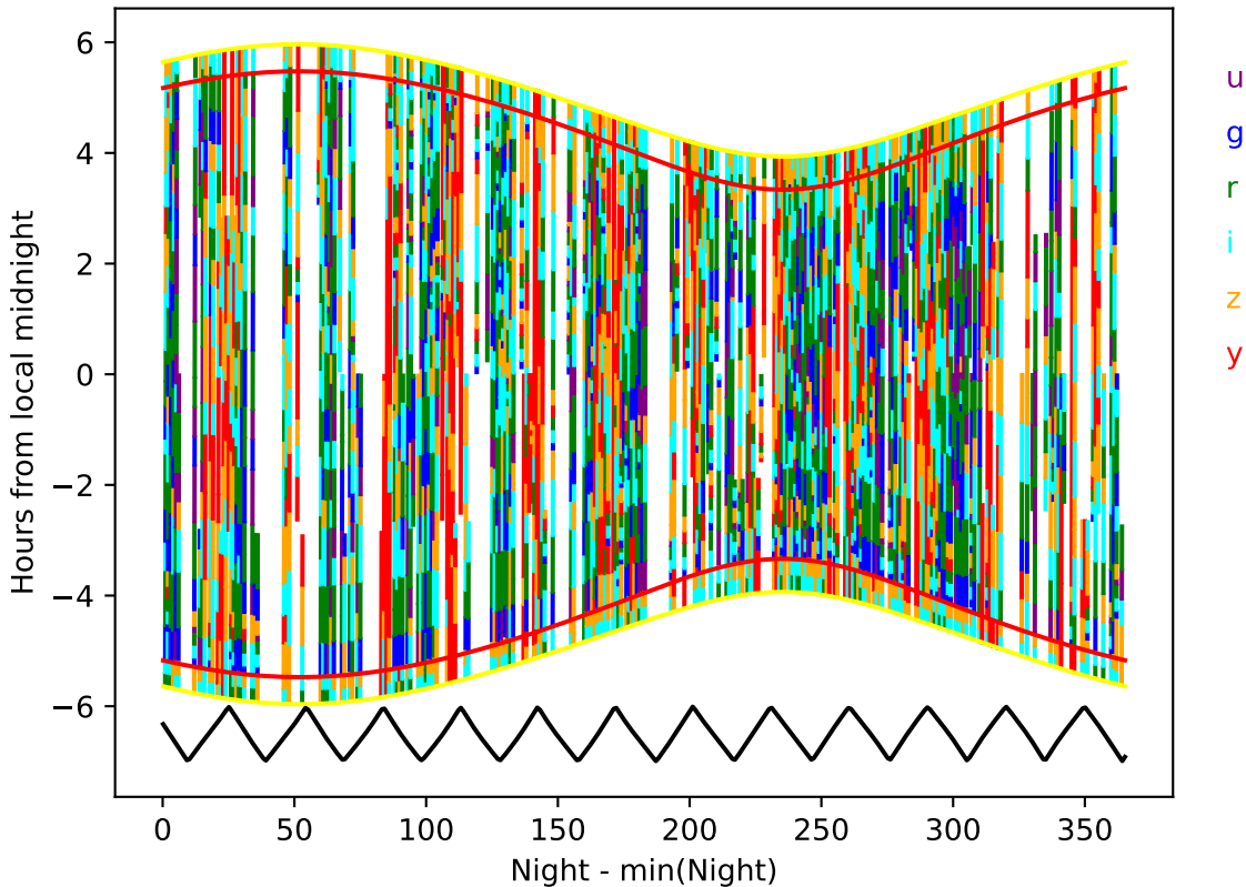
smc_lmc_v3.3_10yrs year 7-8: Hourglass
