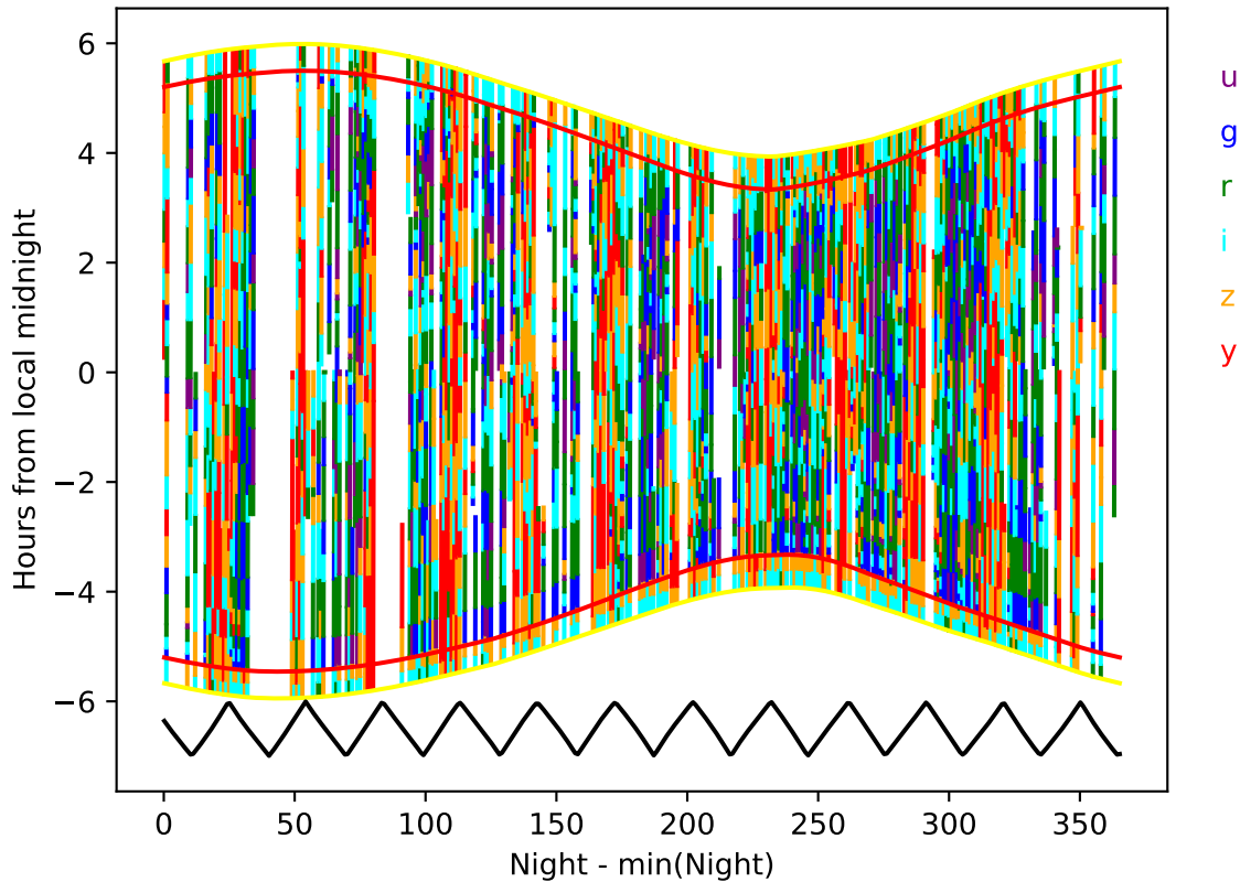
smc_lmc_v3.3_10yrs year 4-5: Hourglass
