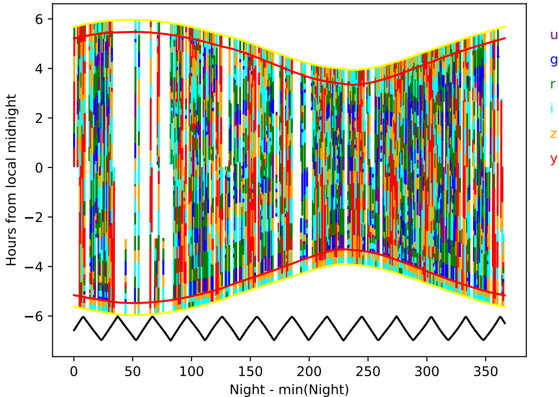
smc_lmc_v3.3_10yrs year 3-4: Hourglass
