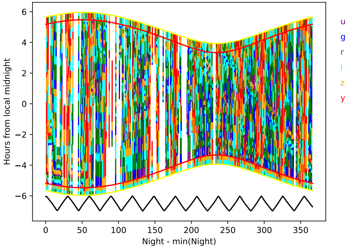
smc_lmc_v3.3_10yrs year 1-2: Hourglass
