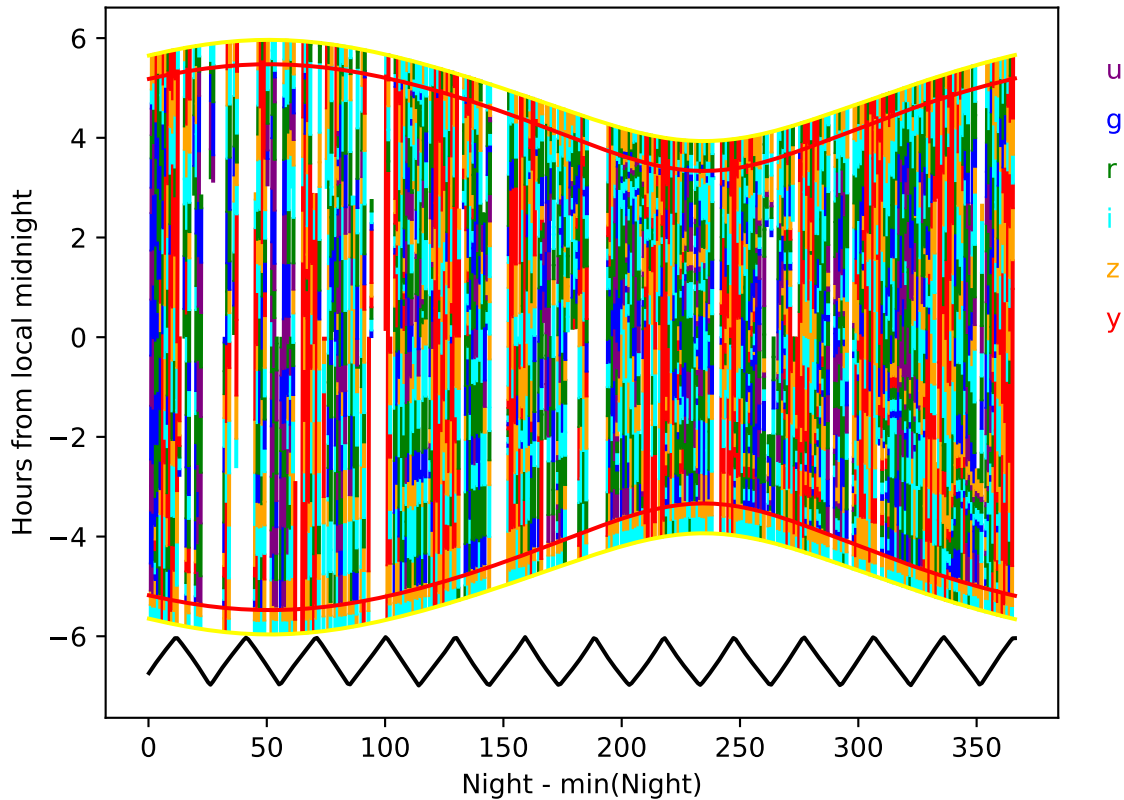
smc_lmc_v3.3_10yrs year 0-1: Hourglass
