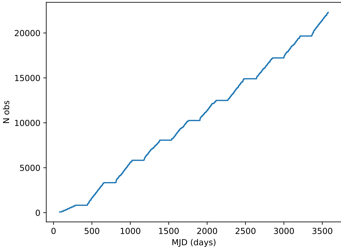
smc_lmc_v3.3_10yrs note like DD:XMM_LSS%: Cumulative
