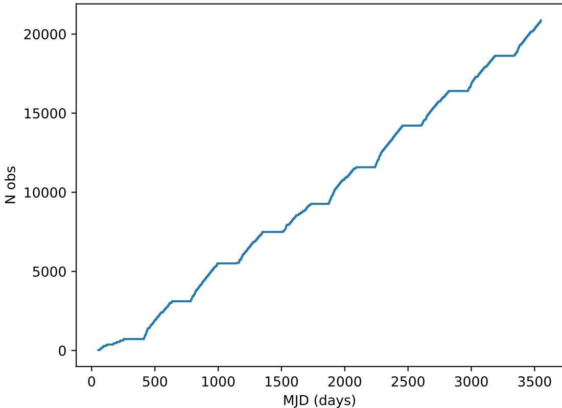
smc_lmc_v3.3_10yrs note like DD:ELAISS1%: Cumulative
