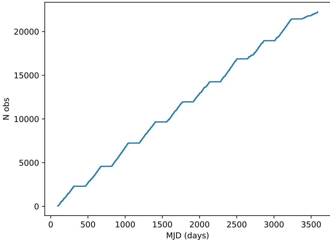
smc_lmc_v3.3_10yrs note like DD:ECDFS%: Cumulative
