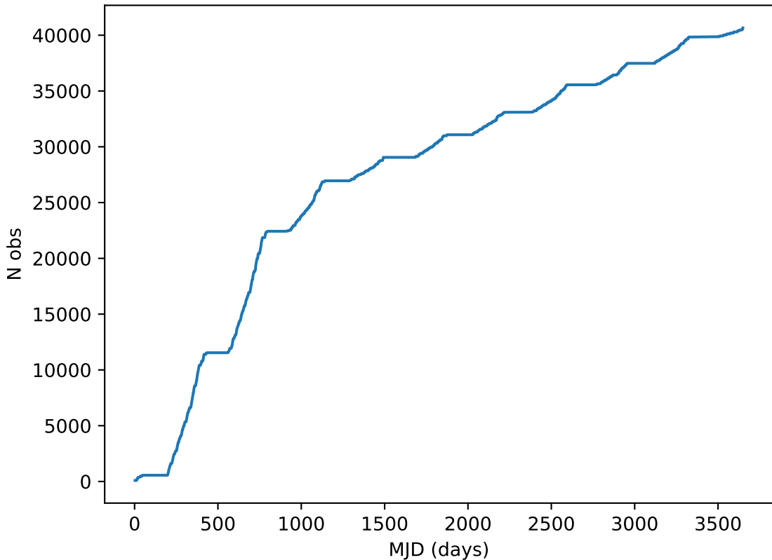
smc_lmc_v3.3_10yrs note like DD:COSMOS%: Cumulative
