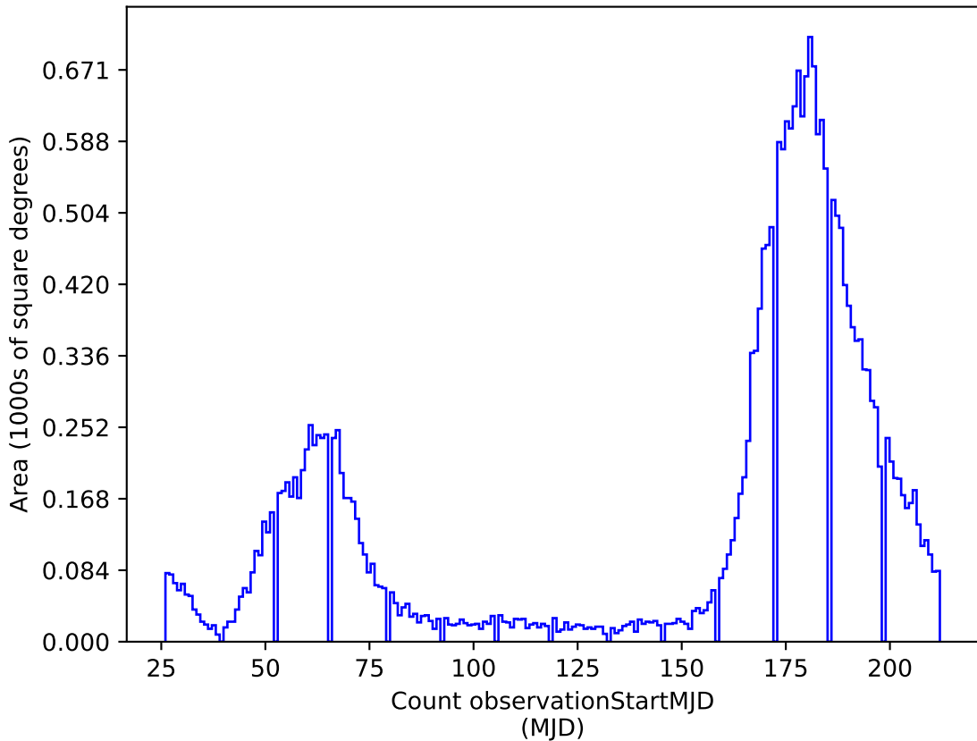
smc_lmc_v3.3_10yrs r: Count observationStartMJD
