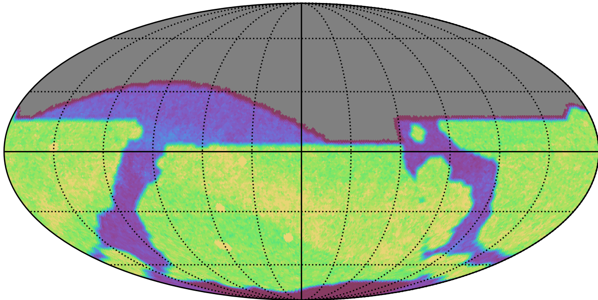
smc_lmc_v3.3_10yrs i: Count observationStartMJD
