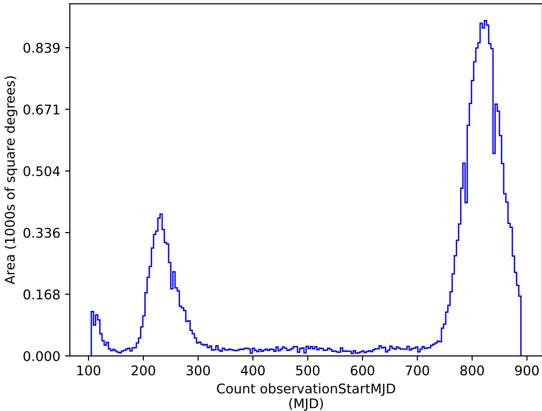
smc_lmc_v3.3_10yrs : Count observationStartMJD
