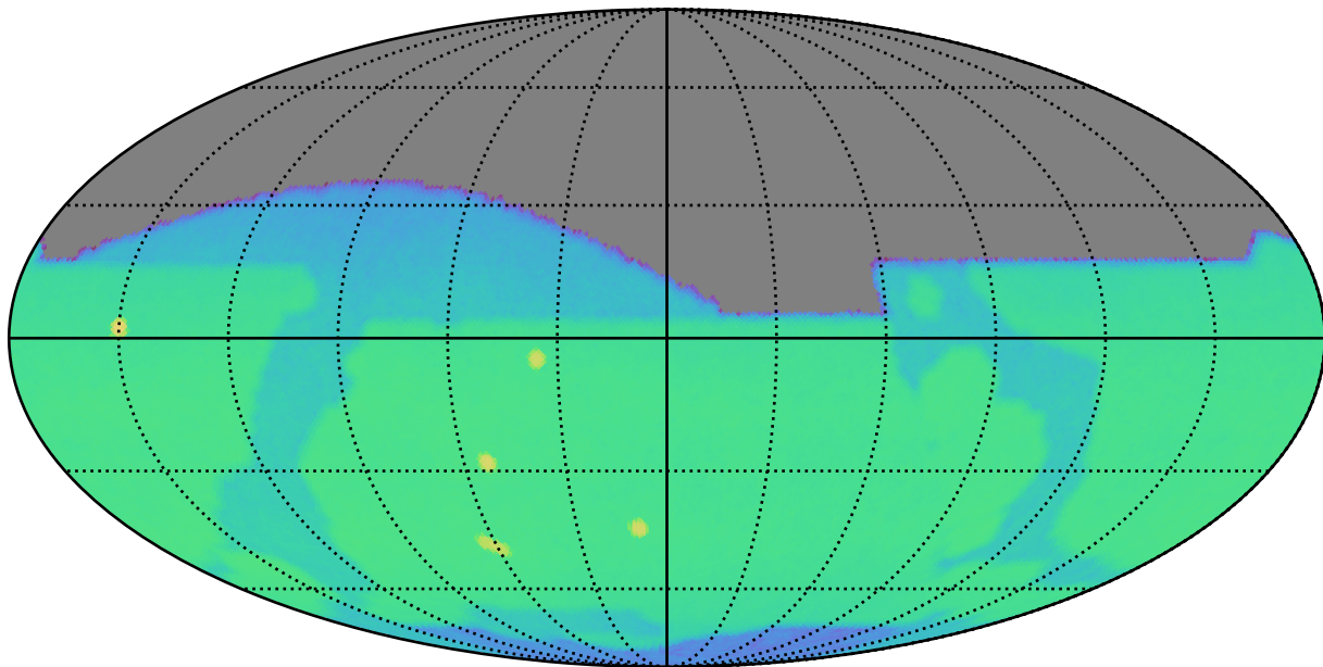
smc_lmc_v3.3_10yrs z: CoaddM5
