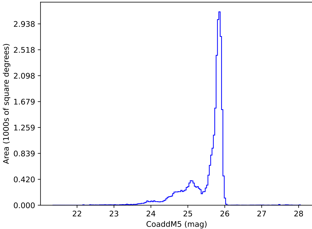
smc_lmc_v3.3_10yrs z: CoaddM5
