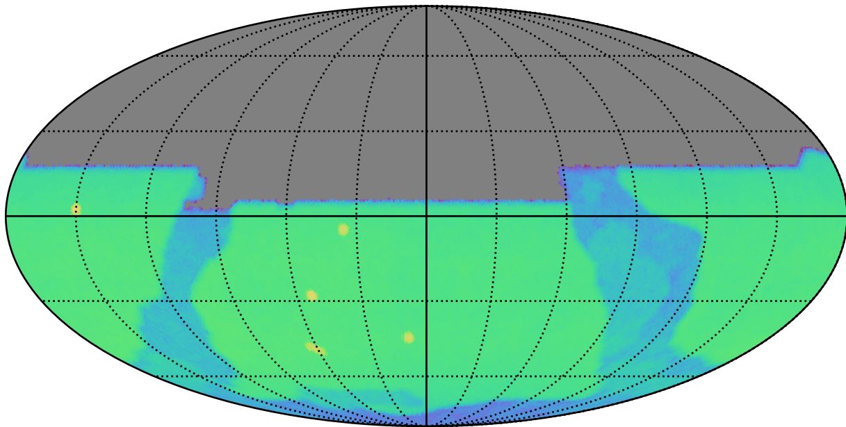
smc_lmc_v3.3_10yrs y: CoaddM5
