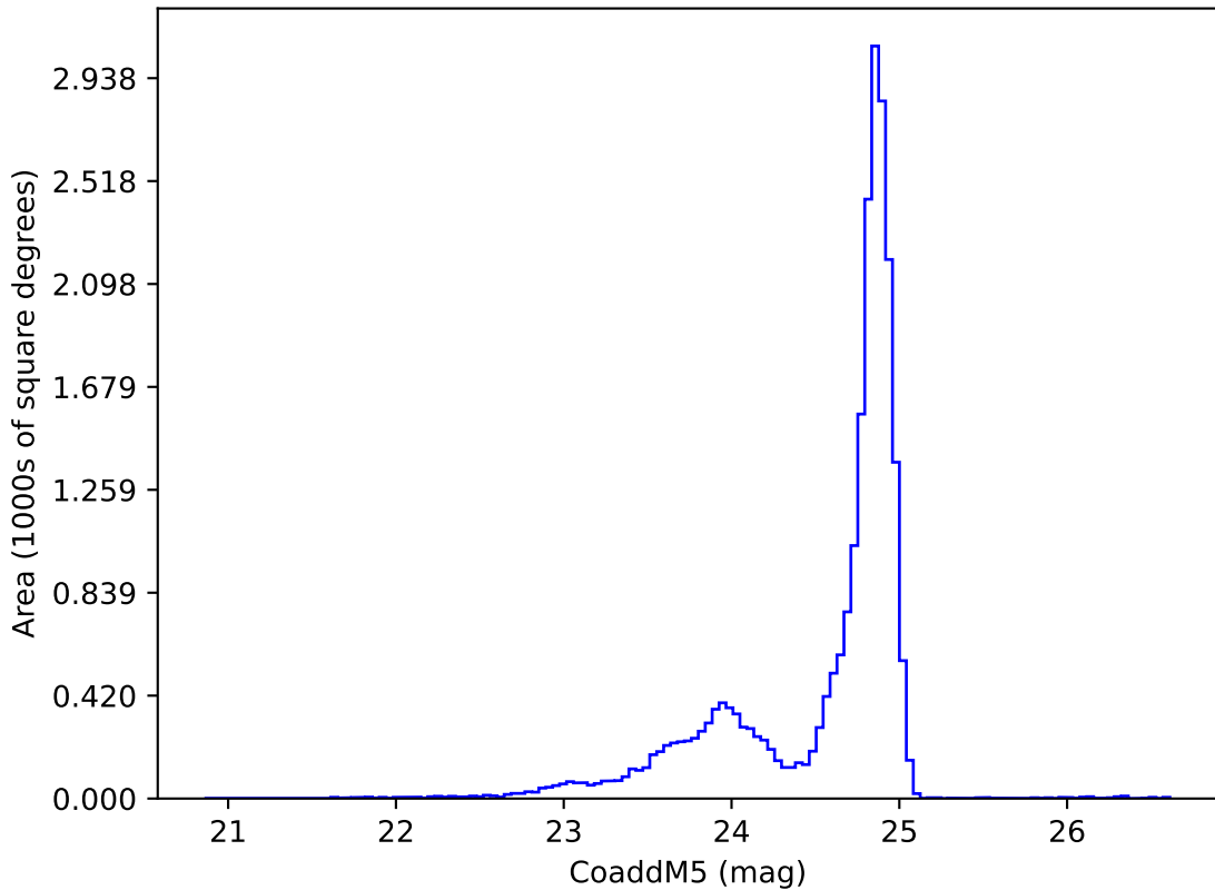
smc_lmc_v3.3_10yrs y: CoaddM5
