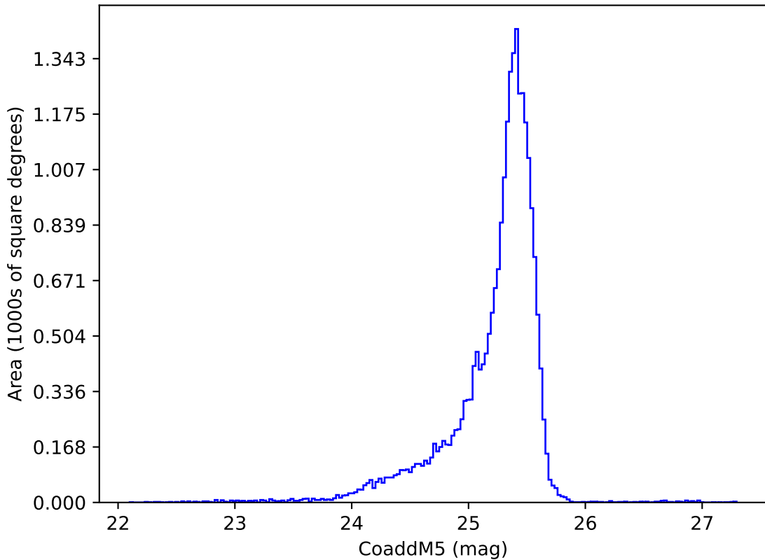
smc_lmc_v3.3_10yrs u: CoaddM5
