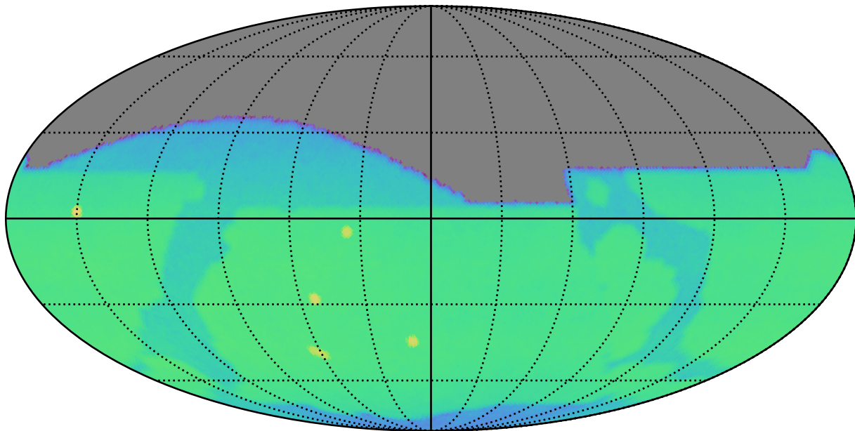
smc_lmc_v3.3_10yrs r: CoaddM5
