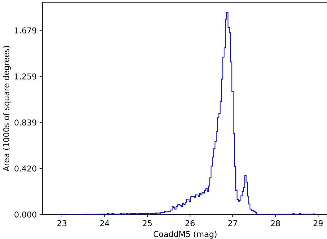
smc_lmc_v3.3_10yrs g: CoaddM5
