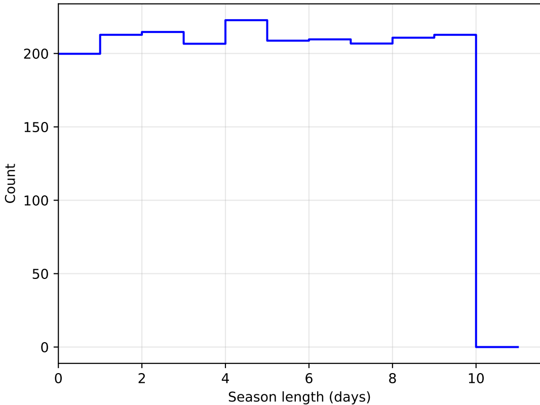
smc_lmc_v3.3_10yrs DD:XMM_LSS all bands: SeasonLength
