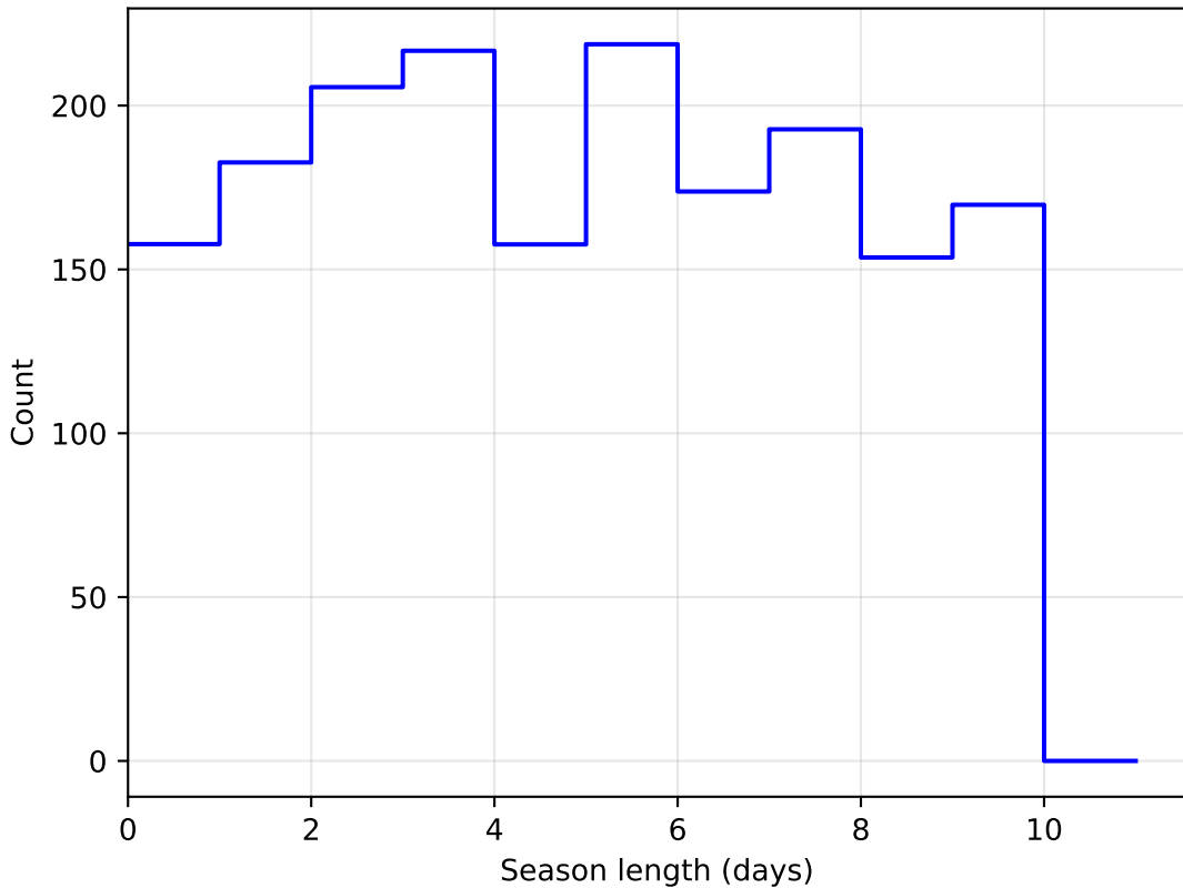
smc_lmc_v3.3_10yrs DD:WFD all bands: SeasonLength
